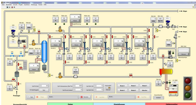
Flow sheet of a multi-stage gas permeation plant.
