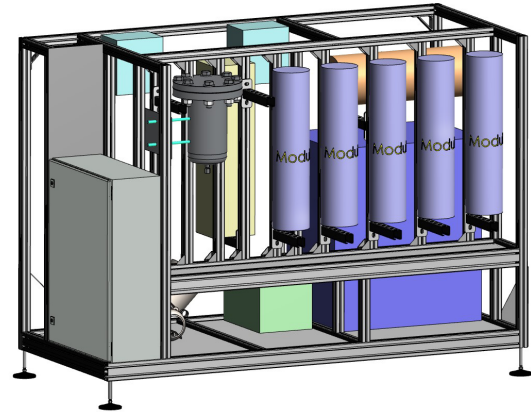
3D layout of gas permeation plant.
