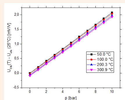
Characteristic curve of a 10 bar relative pressure sensor
